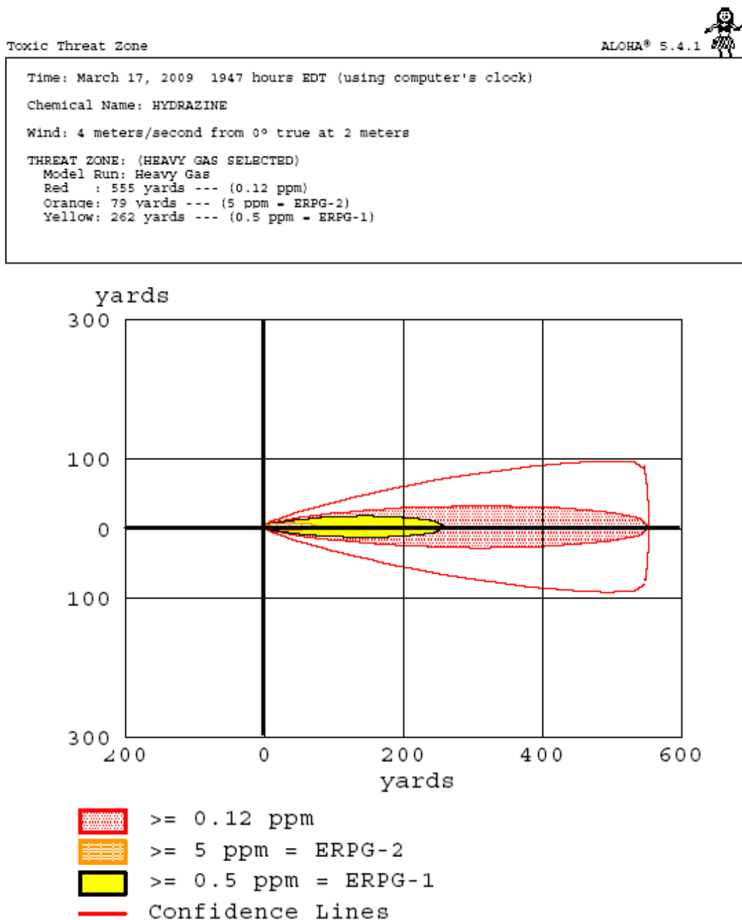
Appendix A Figure 1: Example Threat Zone Plot in ALOHA Model
