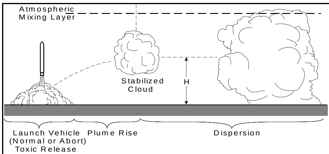
Appendix B Figure 2. Conceptual Illustration of Rocket Exhaust Source Cloud Formation, Cloud Rise and Cloud Atmospheric Dispersion (NASA, 2009b).
