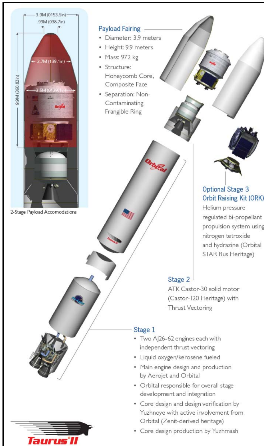
Taurus II Rocket Configuration. Source: Orbital Taurus II Fact Sheet, 2008
