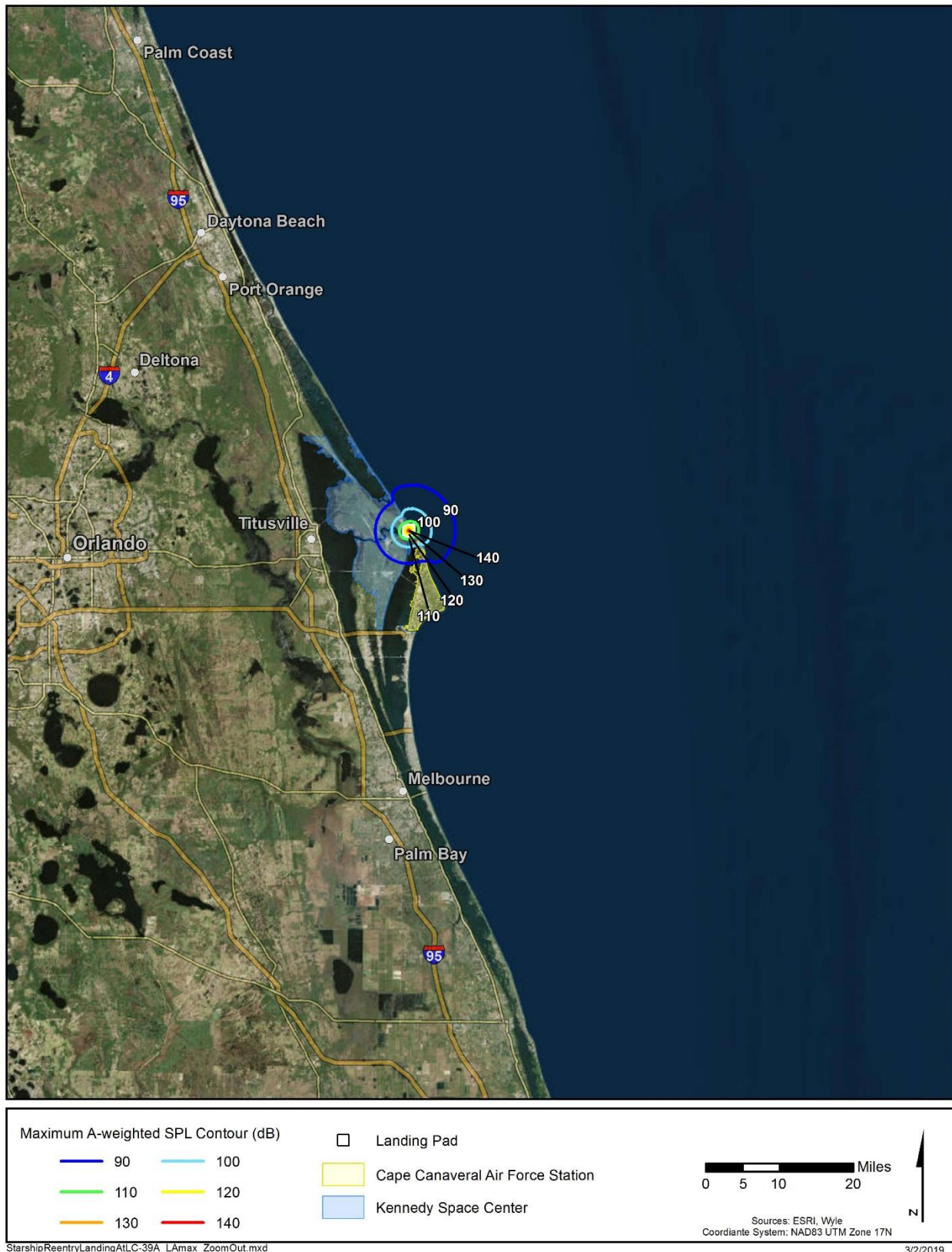
Figure 16. Starship Landing at LC-39A: Maximum A-Weighted Sound Levels
