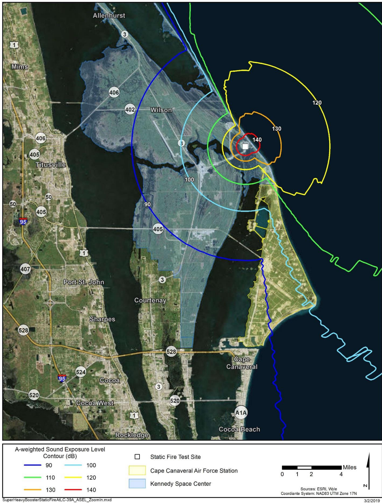
Figure 33. Super Heavy Booster Static Fire Test at LC-39A: Sound Exposure Levels (Zoomed in)
