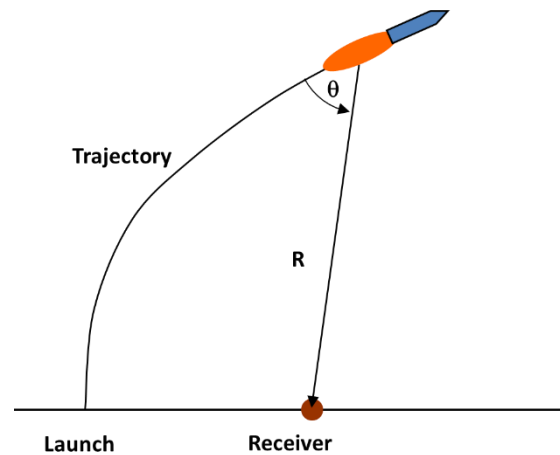
Figure 10. Modeling Rocket Noise at the Ground
