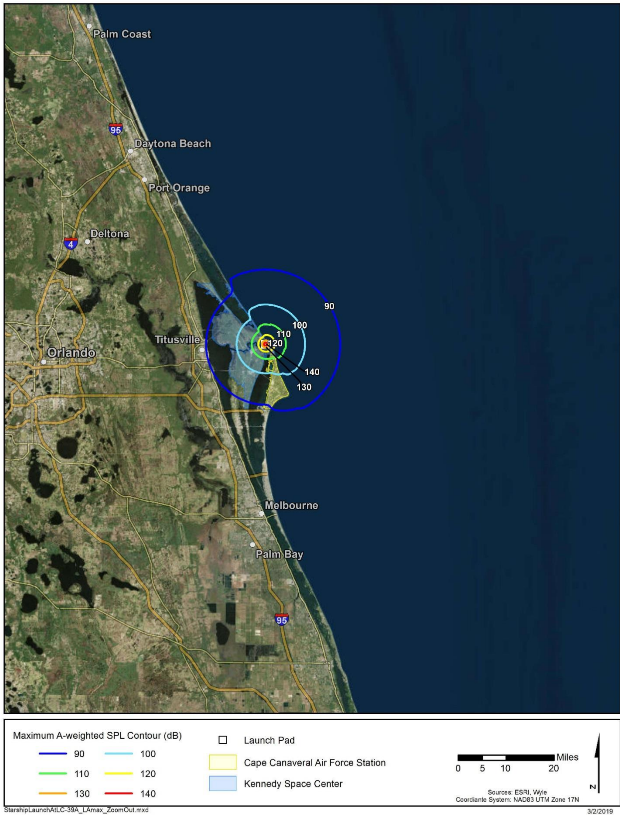
Figure 11. Starship Launch from LC-39A: Maximum A-Weighted Sound Levels
