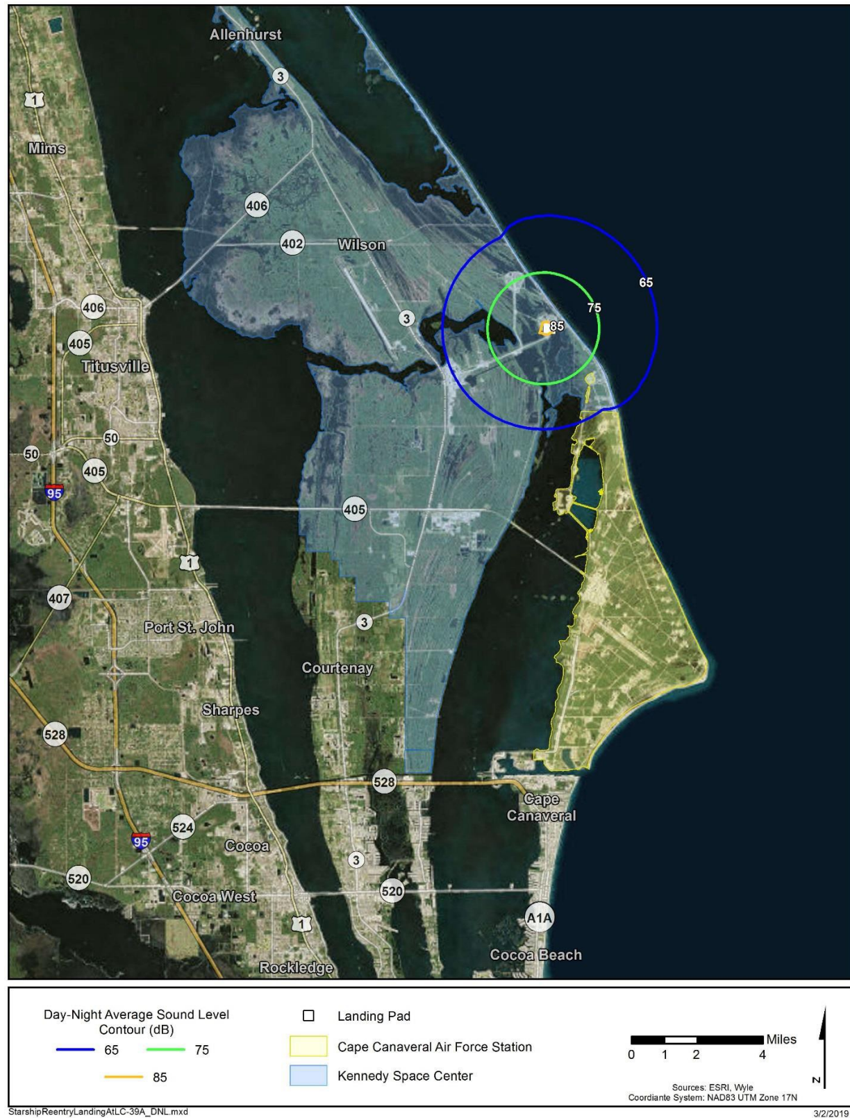
Figure 3-3. Starship Landing at LC-39A: Day-Night Average Sound Levels
