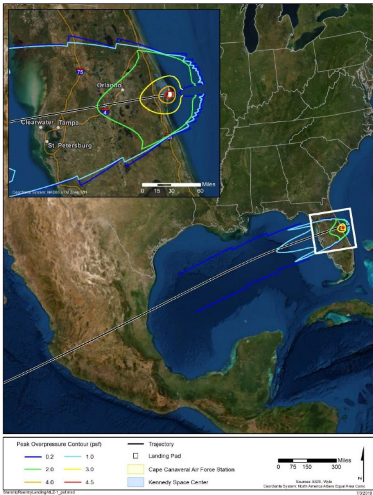
Figure 3-8. Starship Sonic Boom Levels for Reentry/Landing at LZ-1
