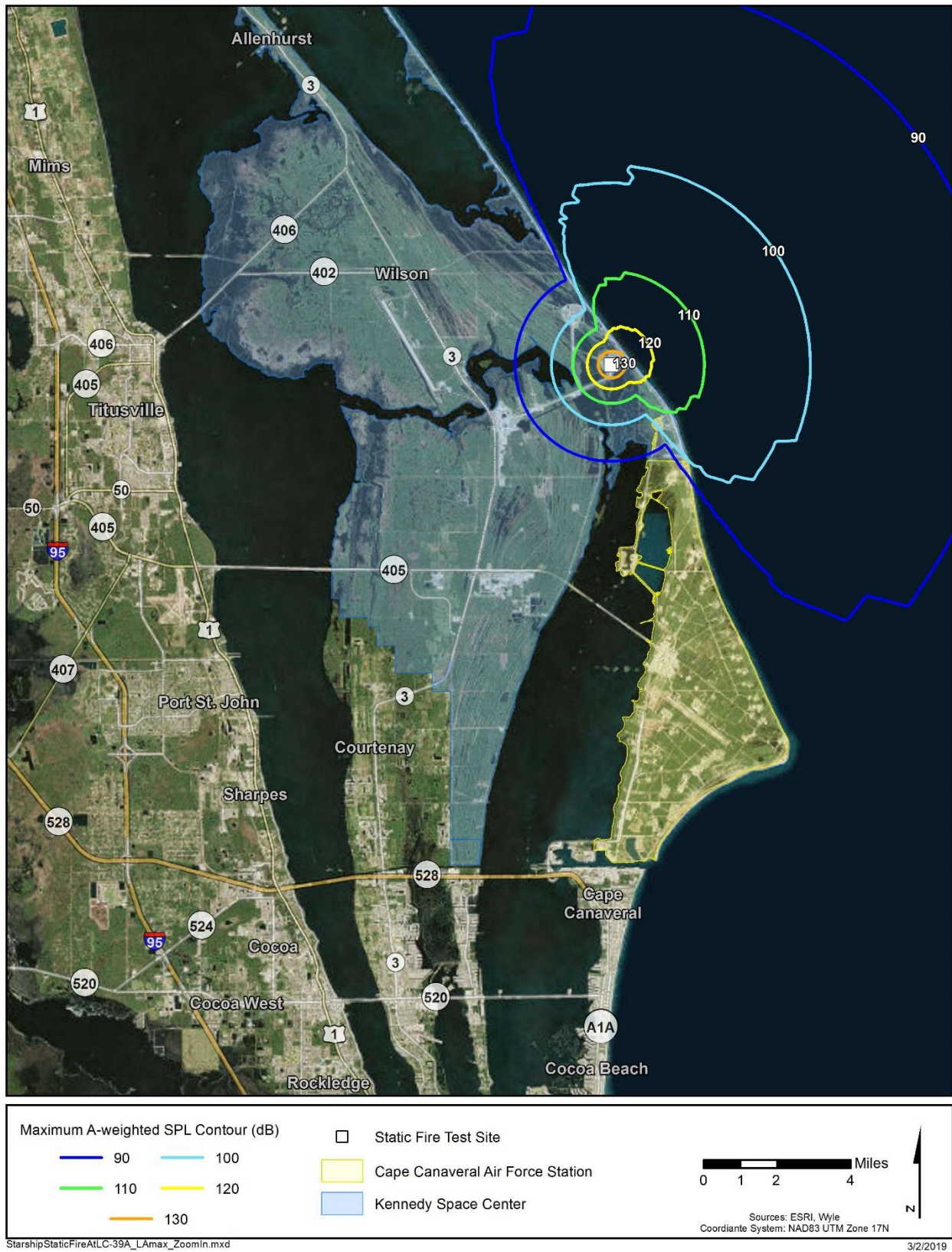
Figure 26. Starship Static Fire Test at LC-39A: Maximum A-Weighted Sound Levels (Zoomed in)
