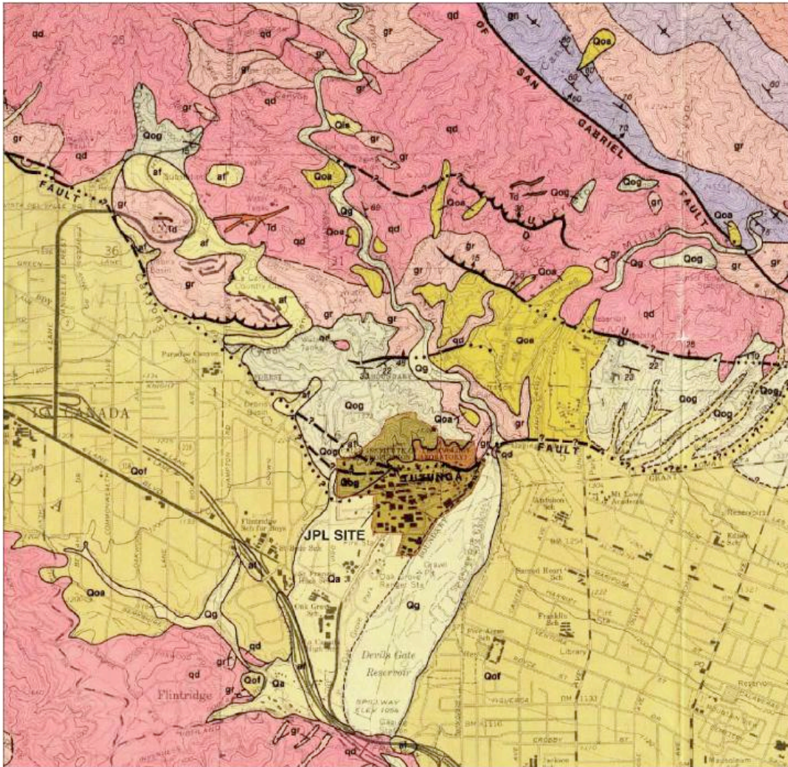
Figure 3-1: Regional Geology Map
