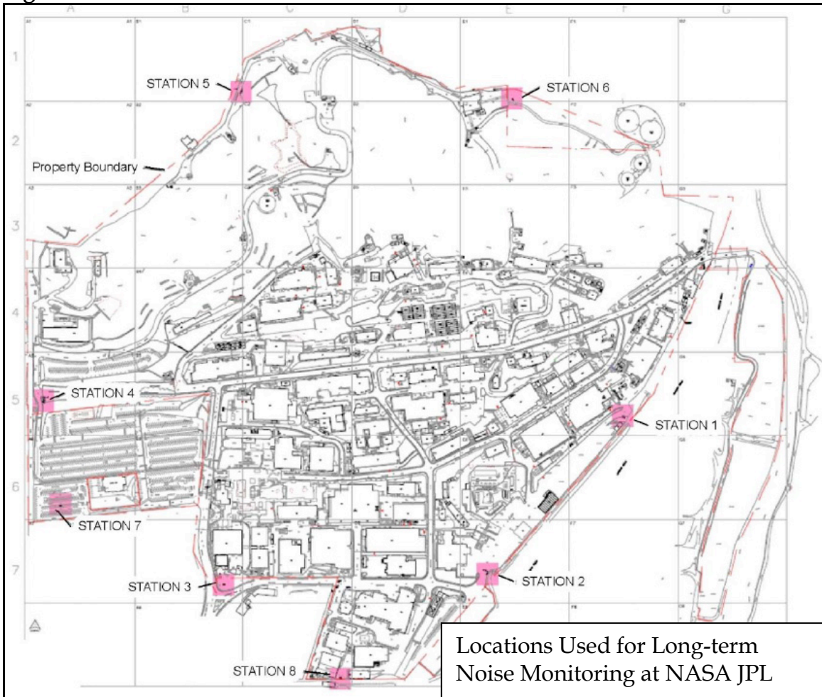
Figure 3-3: Noise Measurement Locations
