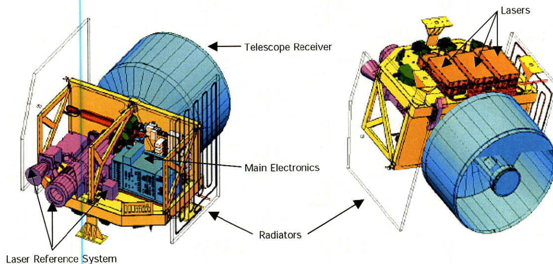
Figure 2-1. Geoscience Laser Altimeter System (GLAS)
